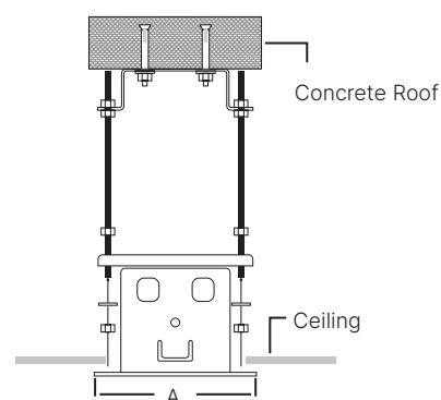
Installation Diagram
