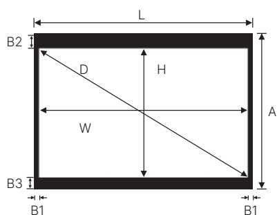
Installation Diagram:
